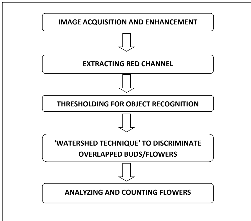
Figure 1. Workflow of the methodology.
